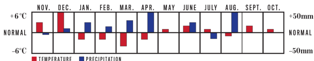
TEMPERATURE AND PRECIPITATION NOVEMBER 2019 TO OCTOBER 2020
